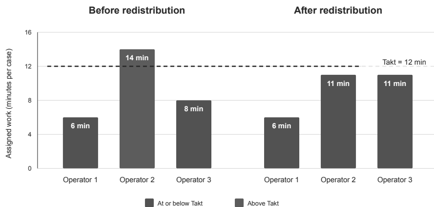
Figure 11.1.: Operator work before and after the proposed redistribution, compared with a 12-minute Takt.
