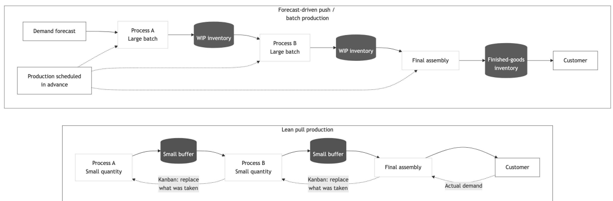
Figure 5.1.: Forecast-driven mass production compared with kanban-controlled pull production.
