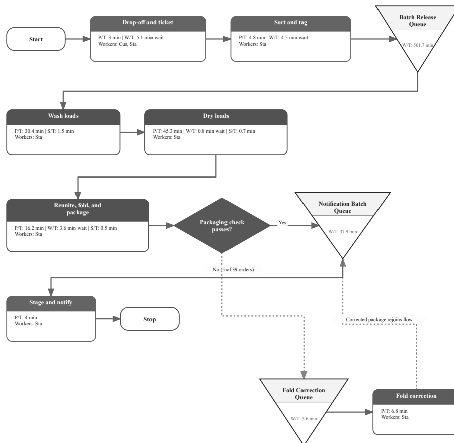
Figure 9.7.: Wash n' Fold current-state map; timing labels state whether their evidence comes from 39 orders, 65 loads, or five correction records.
