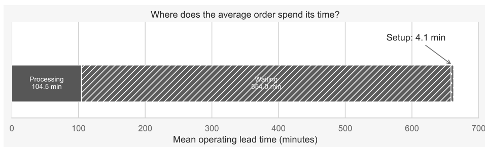
Figure 9.5.: Waiting accounts for most of the mean Wash n' Fold operating lead time.
