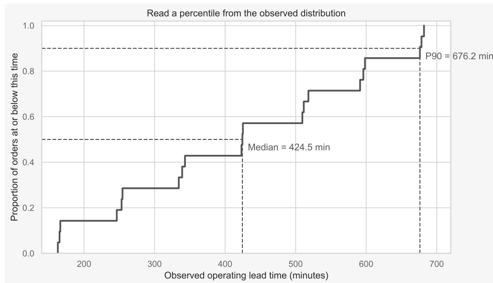
Figure 9.4.: The empirical cumulative distribution connects observed operating lead times to percentiles.
